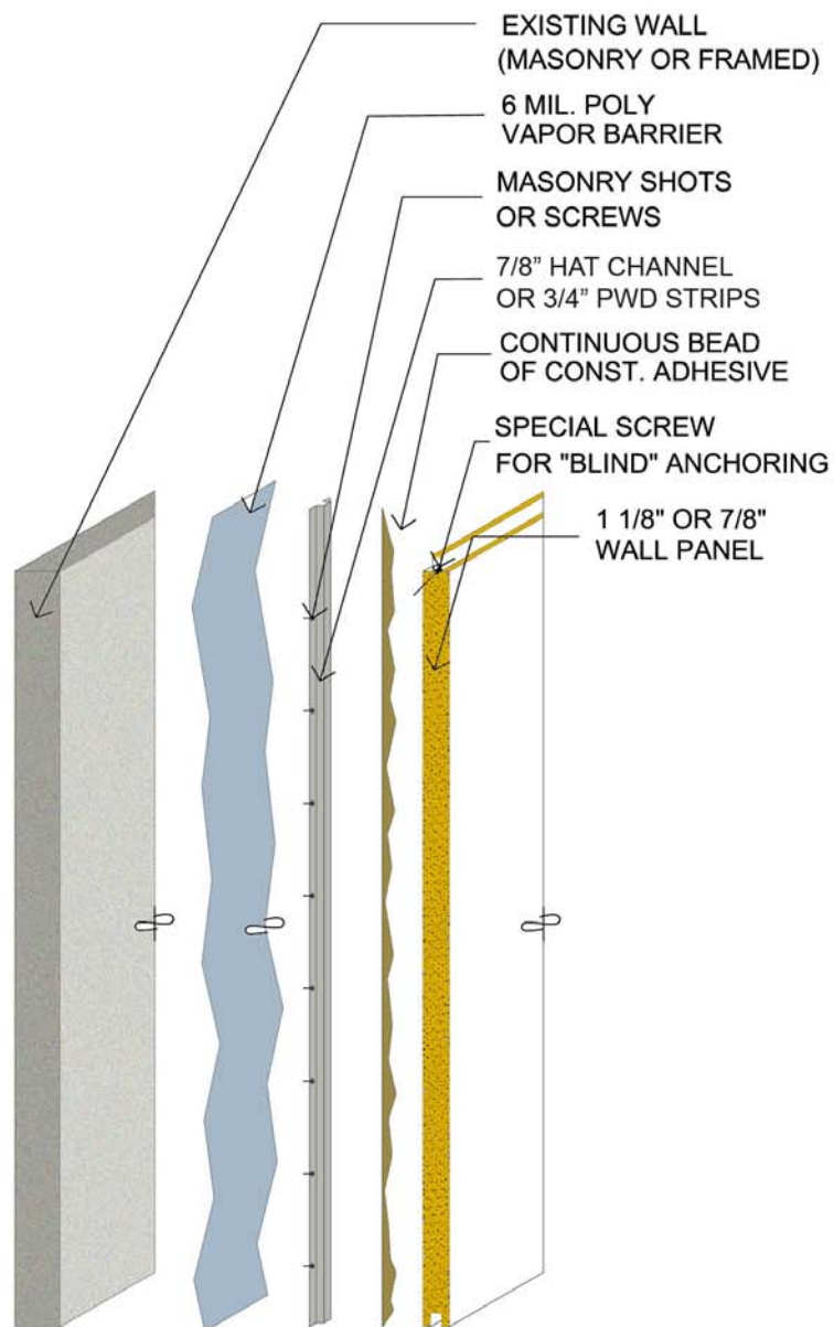
SECTION VIEW
